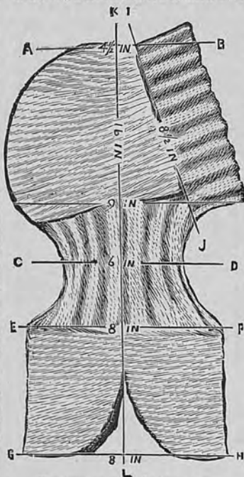
HELMET WHEN COMPLETED.
