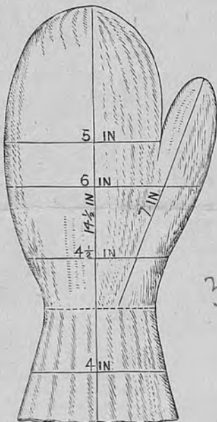
STEERING GLOVE. ( Sea-boot Stocking-yarn, see page 9. )
